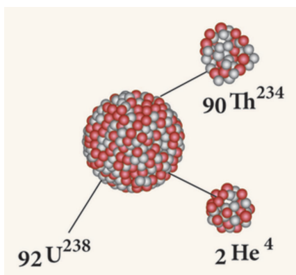
Figure 6.1 Alpha decay
