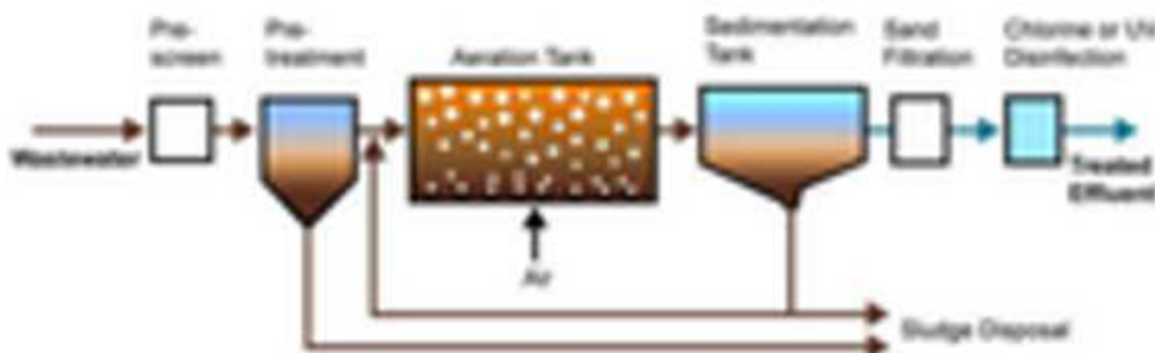
Figure 22.5 Conventional Wastewater Treatment
