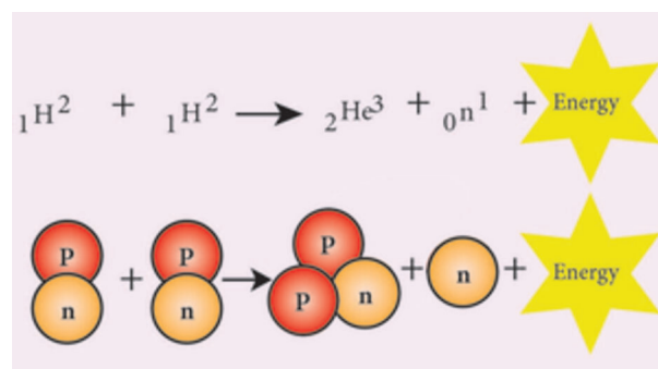
Figure 6.5 Nuclear fusion
