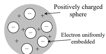
Positive charge spread throughout the sphere
